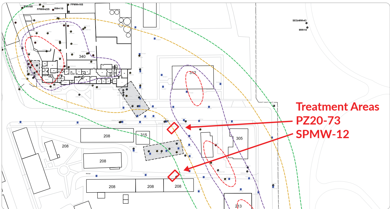
Pilot test treatment areas shown relative to the chlorinated solvent plume.
