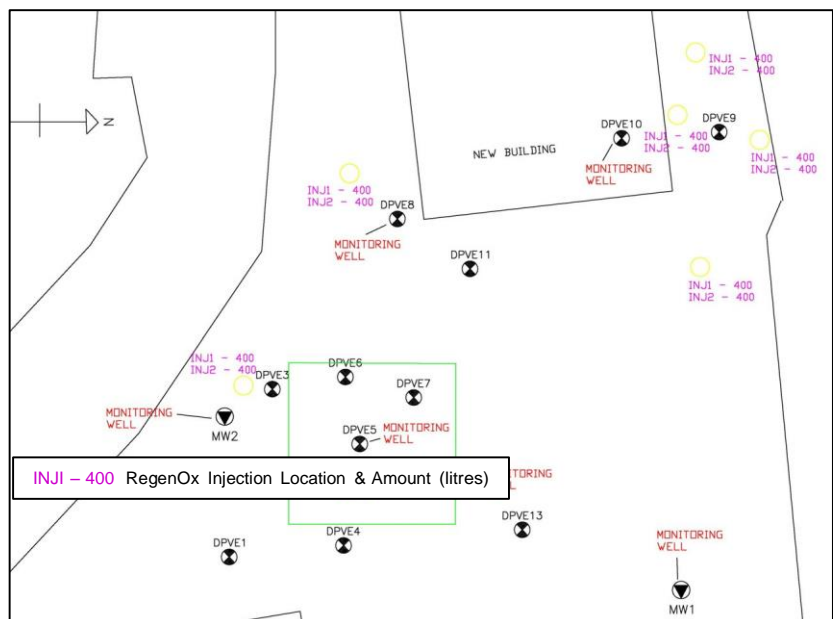
Figure 2. Site Plan Showing RegenOx Locations
