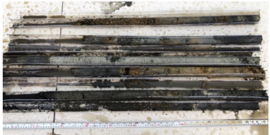
Soil core depicting complete coverage of PlumeStop onto aquifer soil materials.
